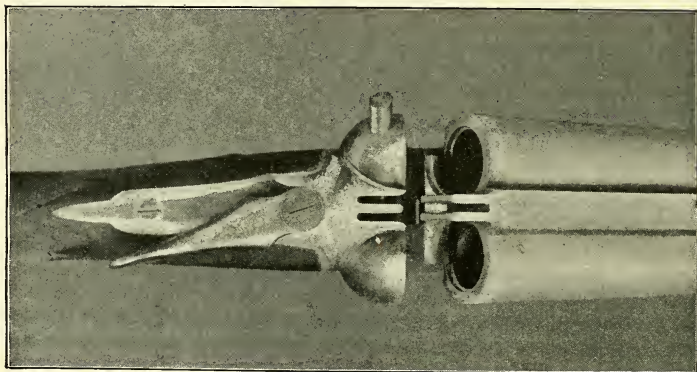
Greener's Improved Wedge-fast Grip.
